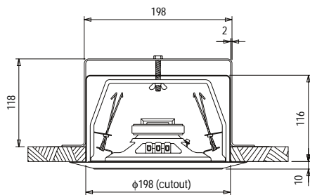
KAS0606WF Side View
