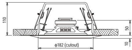
KAS0606W and KAS0610WCOAX Side View
