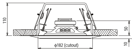
KAS0606W and KAS0610WCOAX Side View
